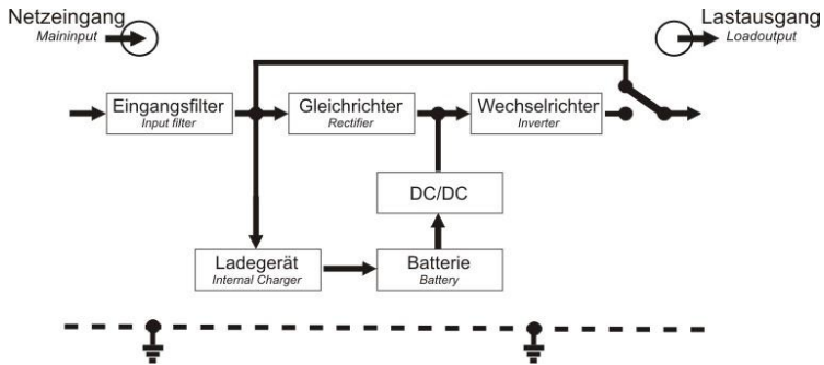
Figure 8: Block diagram
